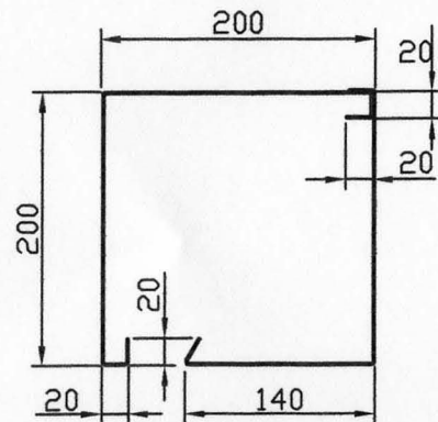
2 OFF SHEET METAL COVER TO SUIT ENDPLATES
